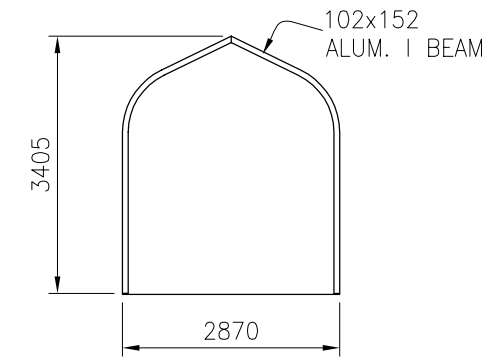
○ SECTION 2.9m HOOD 1:100
