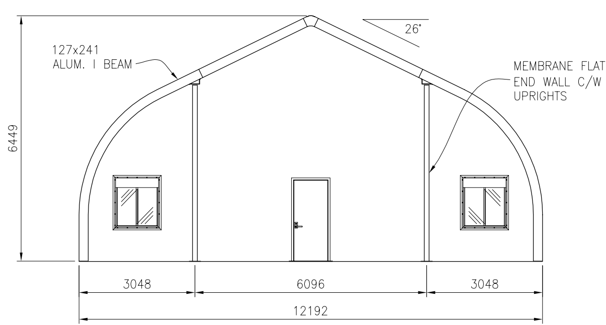
○ FLAT END 12.2m STRUCTURE 1:100
